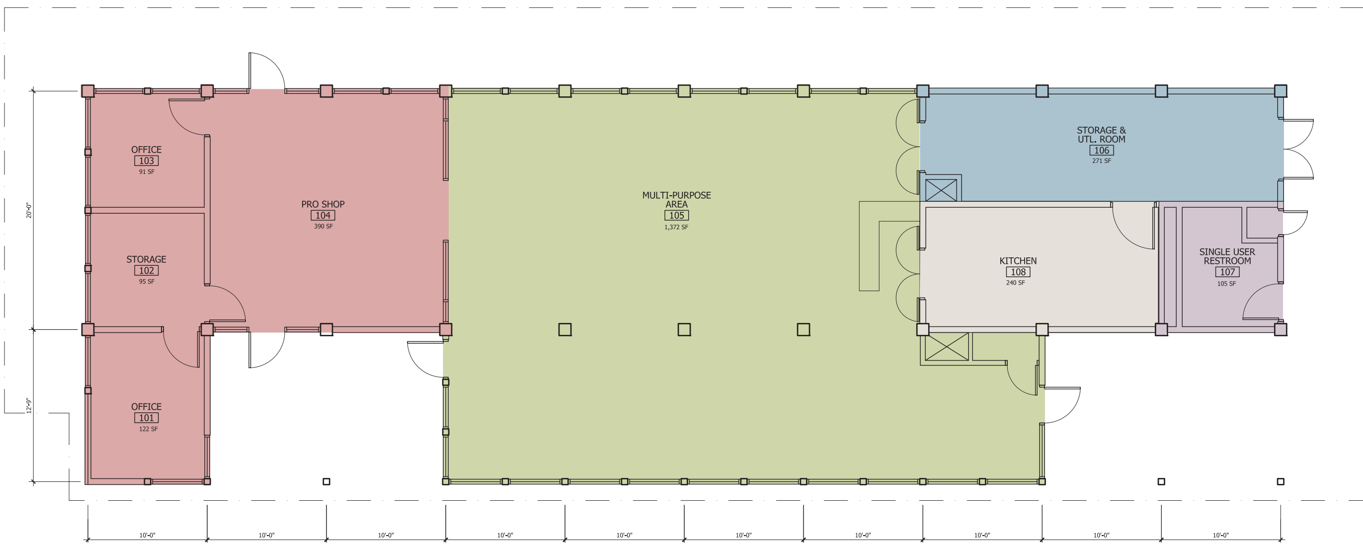
EXISTING FLOOR PLAN - CLUB HOUSE
